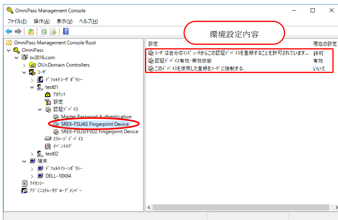
Fig. 3-54 OmniPass Management Console
